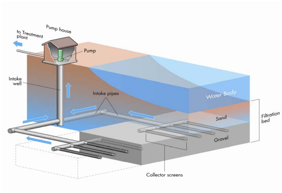
Figure 4-4 – Subsurface Infiltration Gallery (Fukuoka Type Intake)
